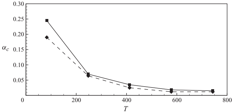
FIGURE 10. Most amplified longitudinal wavenumber versus the target time for Re = 610 , obtained by the direct-adjoint method with L_x = 800 ( \blacklozenge ) and by the superposition of local optimal and suboptimal perturbations ( \blacksquare ).
